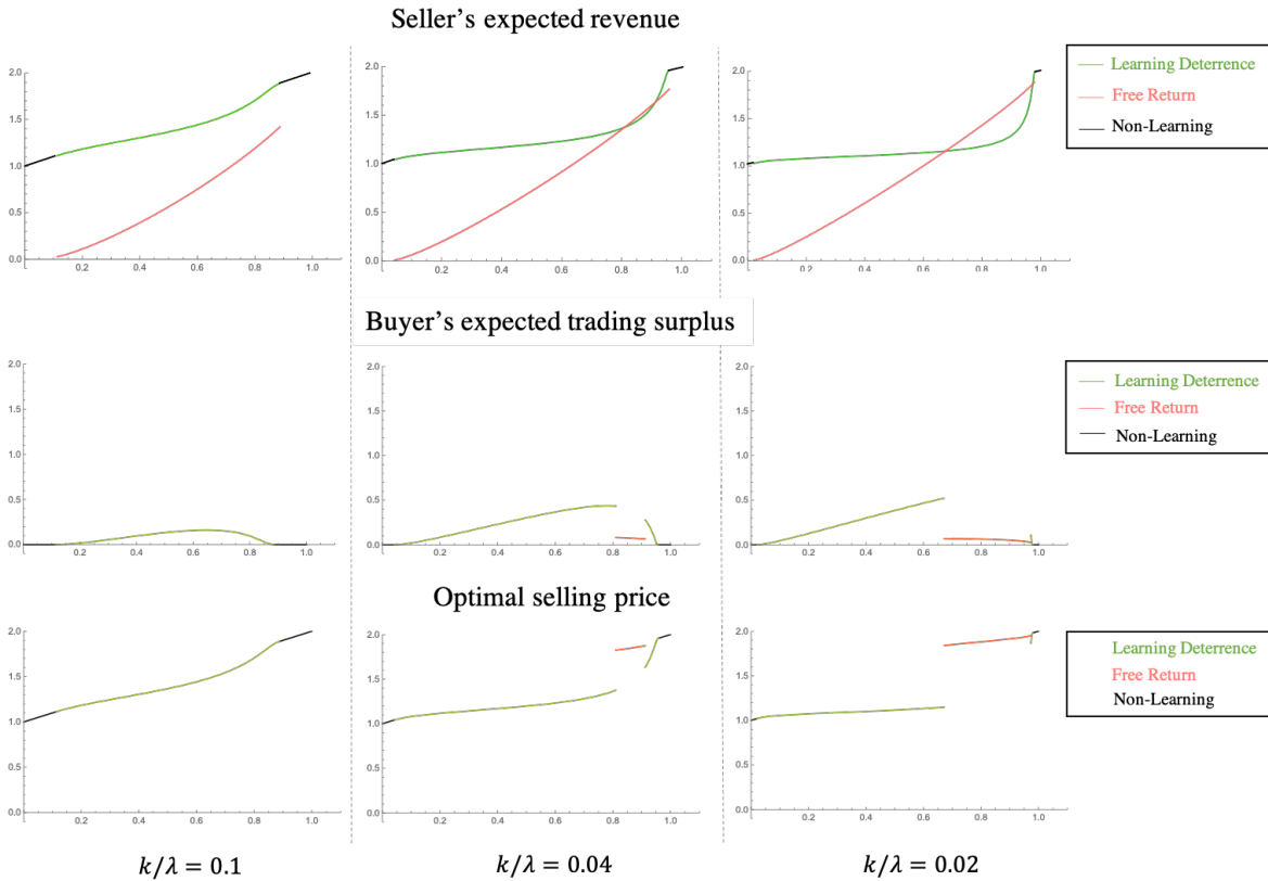
Figure 7: Comparative statics
