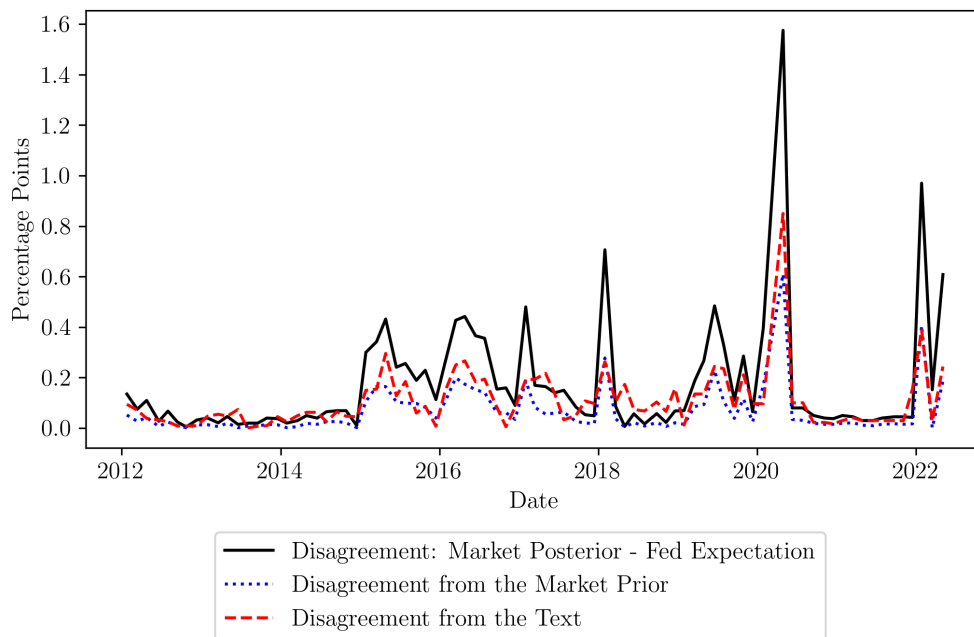
Figure 12: Disagreement Decomposition
