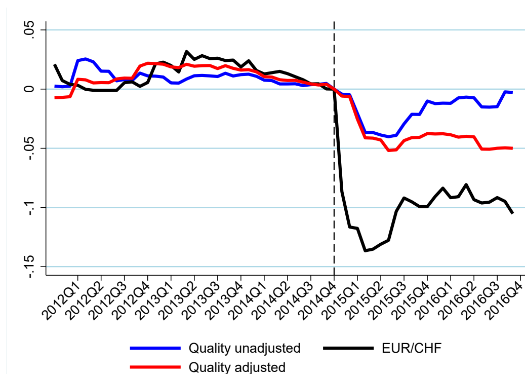
Figure VI.1: Dynamics of the export price index
