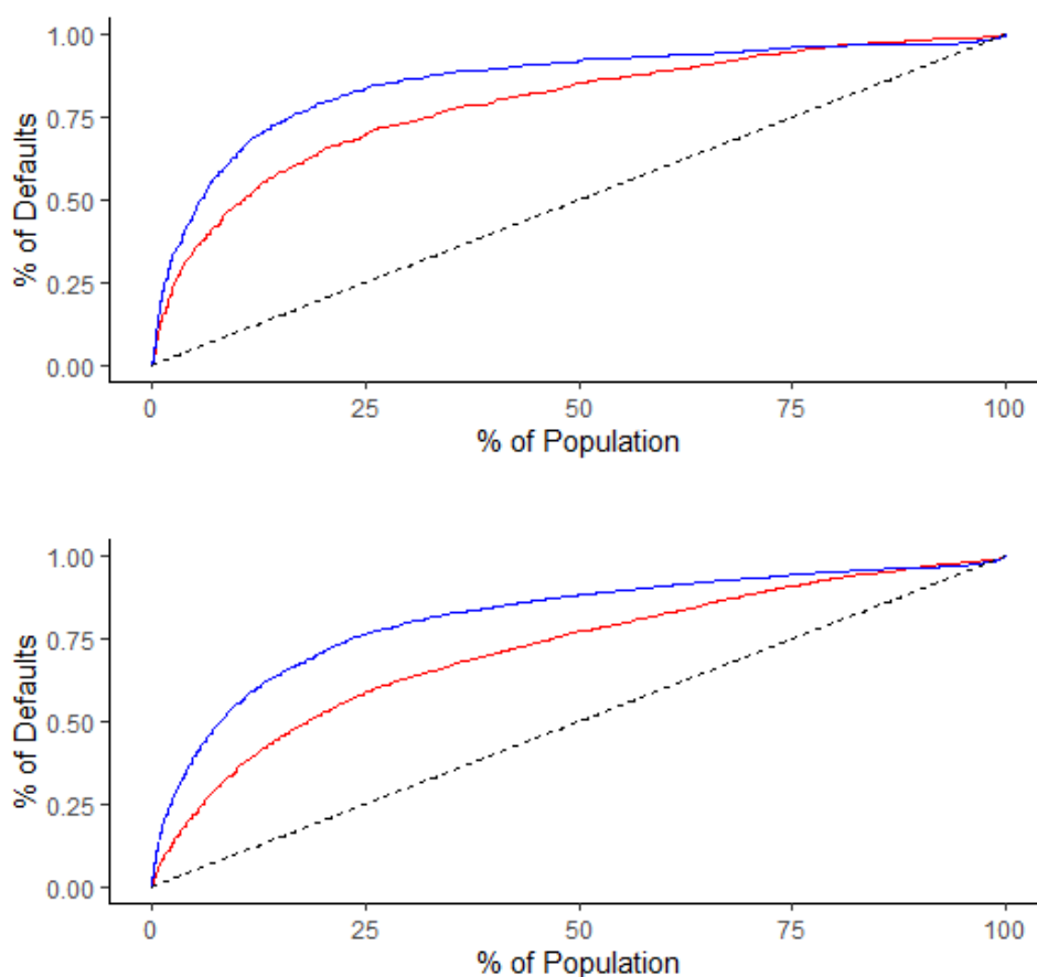
Figure 4: Cumulative Accuracy Paths (3- and 12-month ahead)
