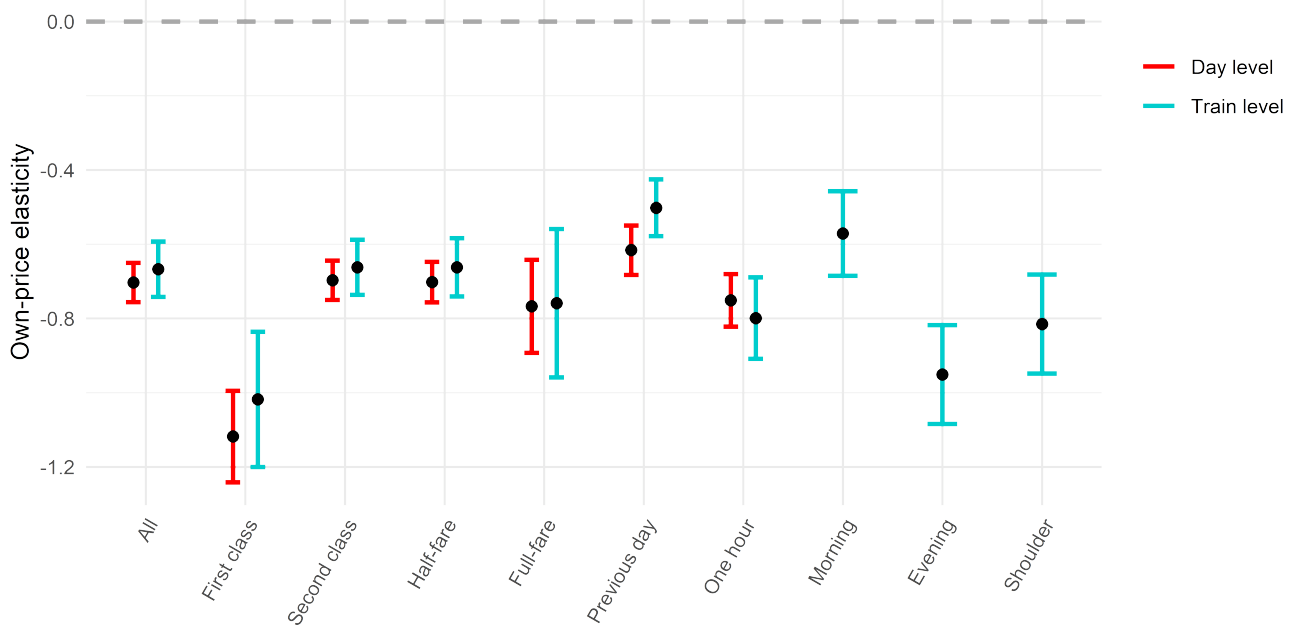
Figure 4: Own-price elasticity for the full sample and different subsets
