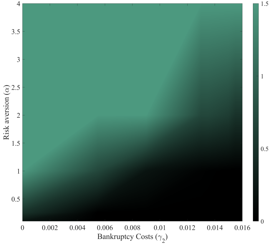
Figure 7. Heatmap of optimal interbank connectivity
