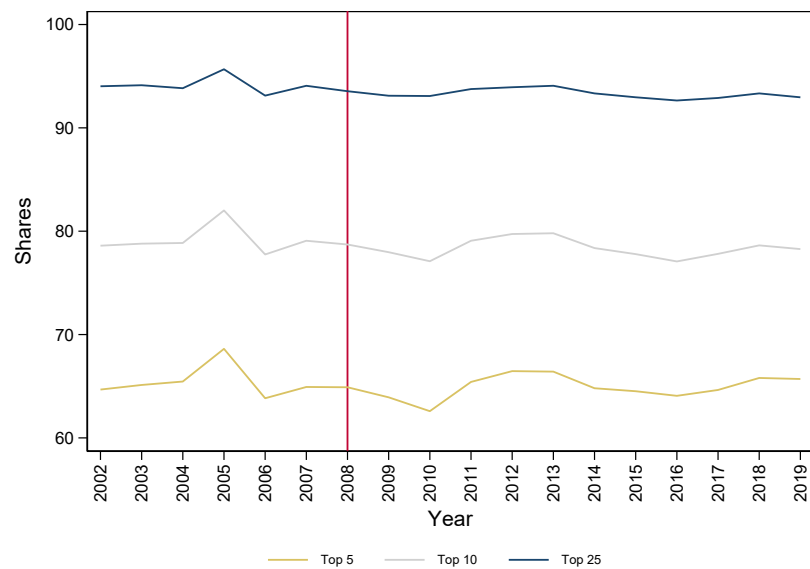
Figure 3.4: Top shares
