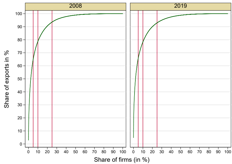
Figure 3.3: Cumulative distribution
