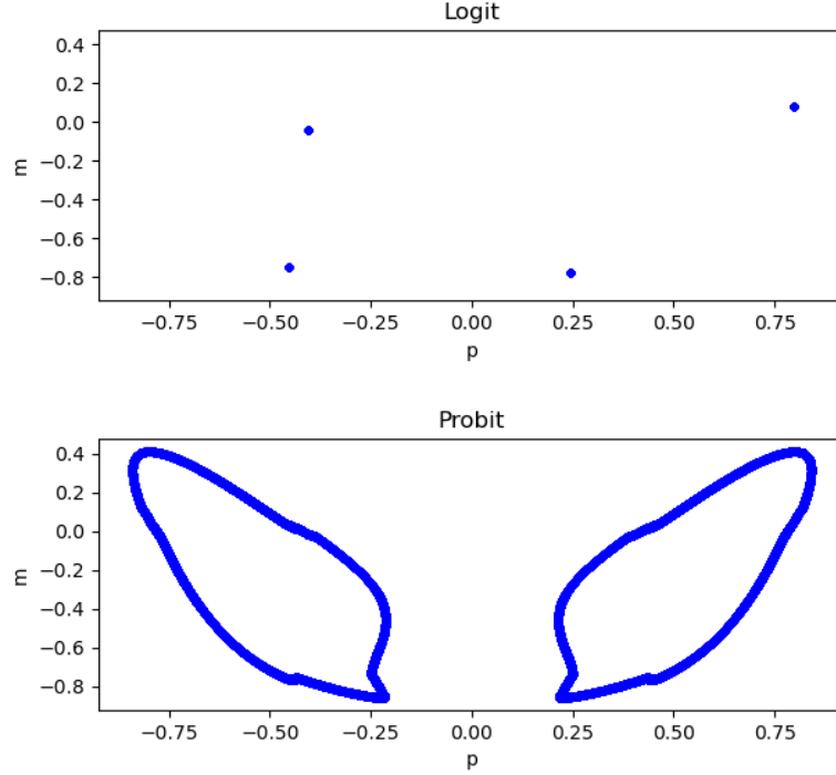
Figure 8: Strange attractor and 4-cycle in P, m -plane
