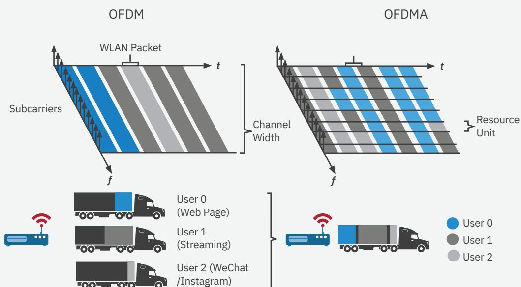
Figure A3: OFDM versus OFDMA
