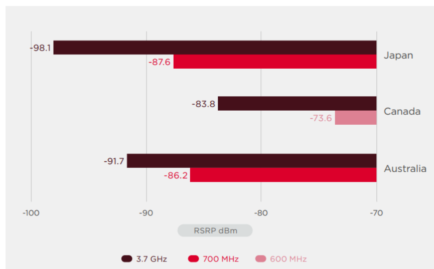
Figure 5: Indoor signal strength using low- and mid-band spectrum, Q3 2022
