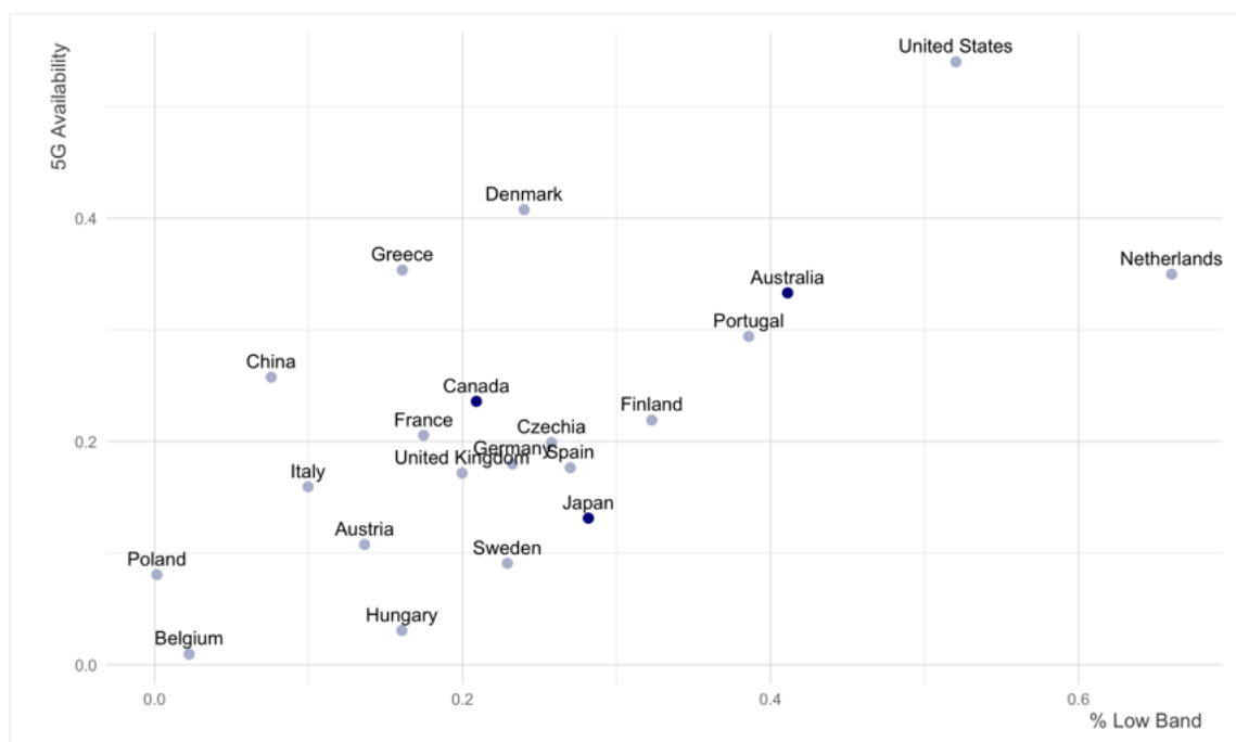
Figure 4: 5G availability and use of low-band, Q3 2022
