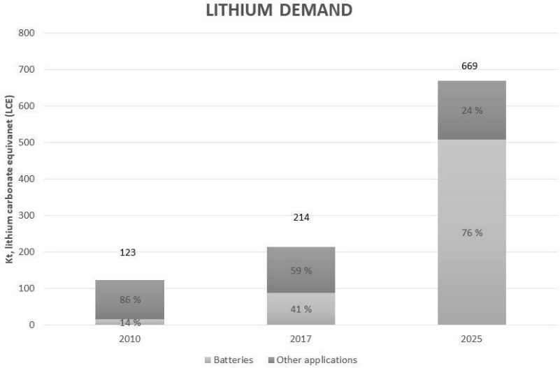
Figure 3 Evolution of lithium demand split by battery sector and other applications
