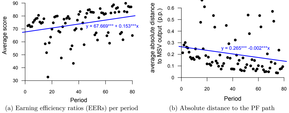
Figure 3: Convergence and learning in the experiment
