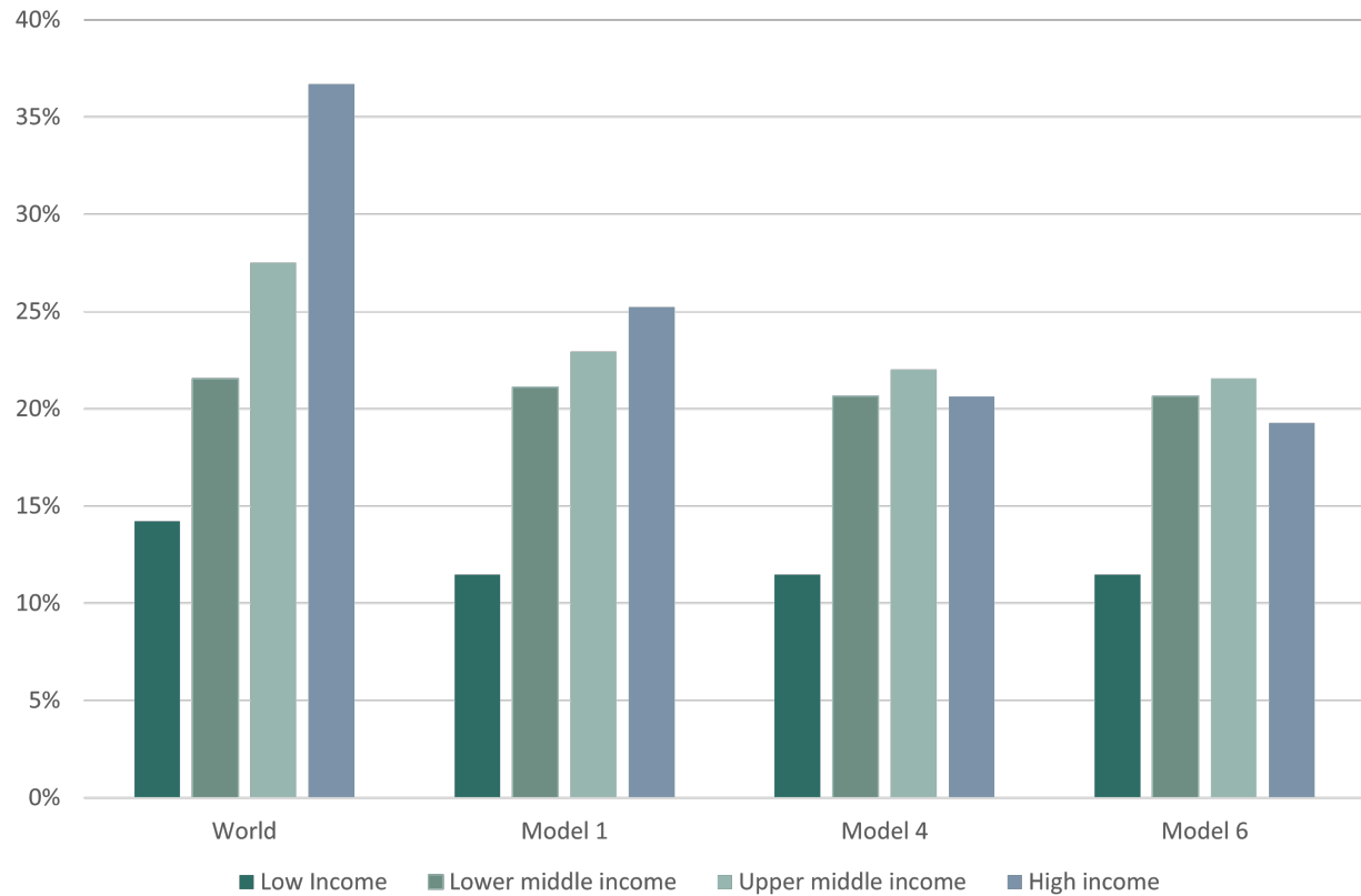
Figure 9: Data selection.
