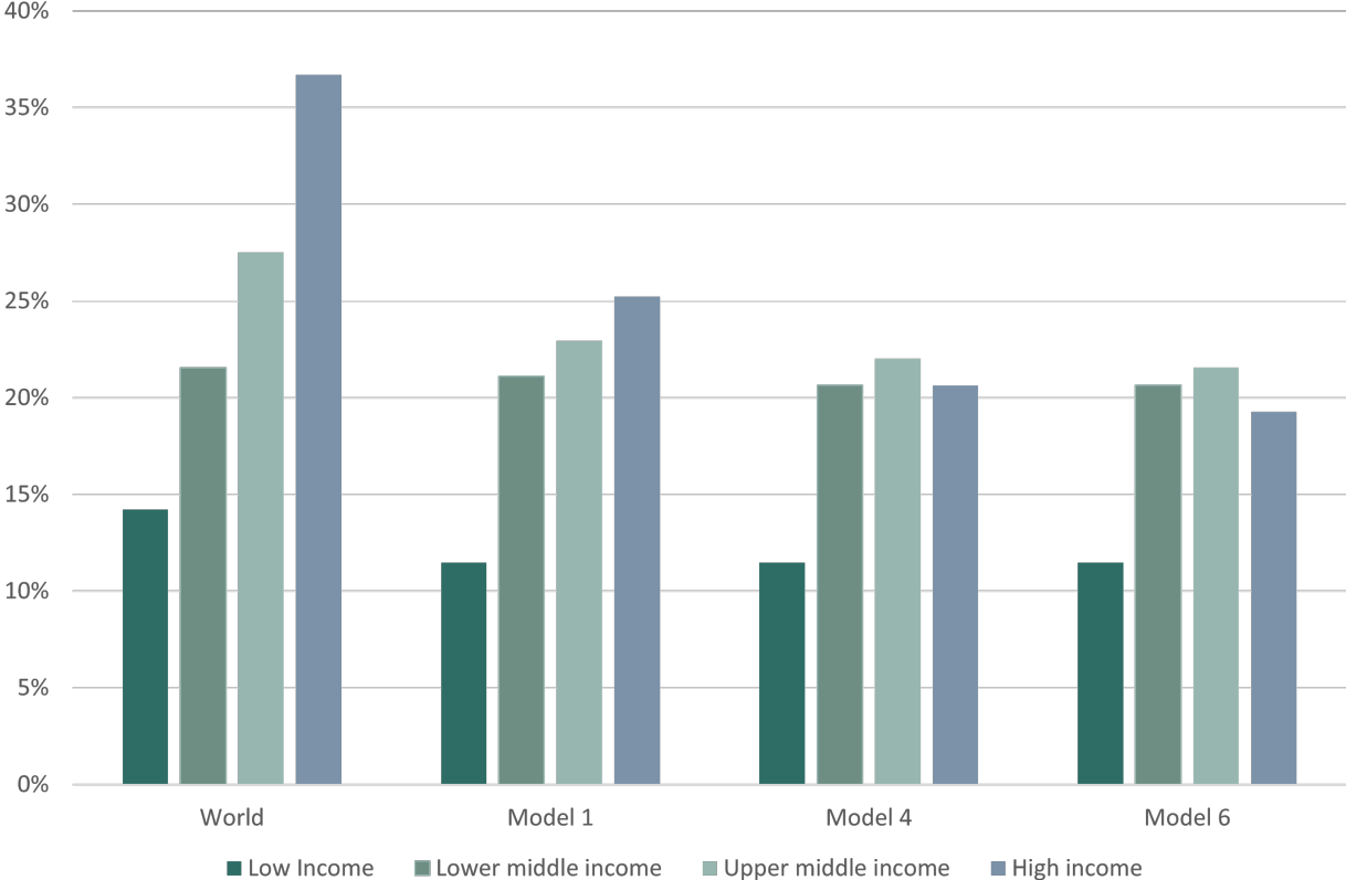
Figure 9: Data selection.
