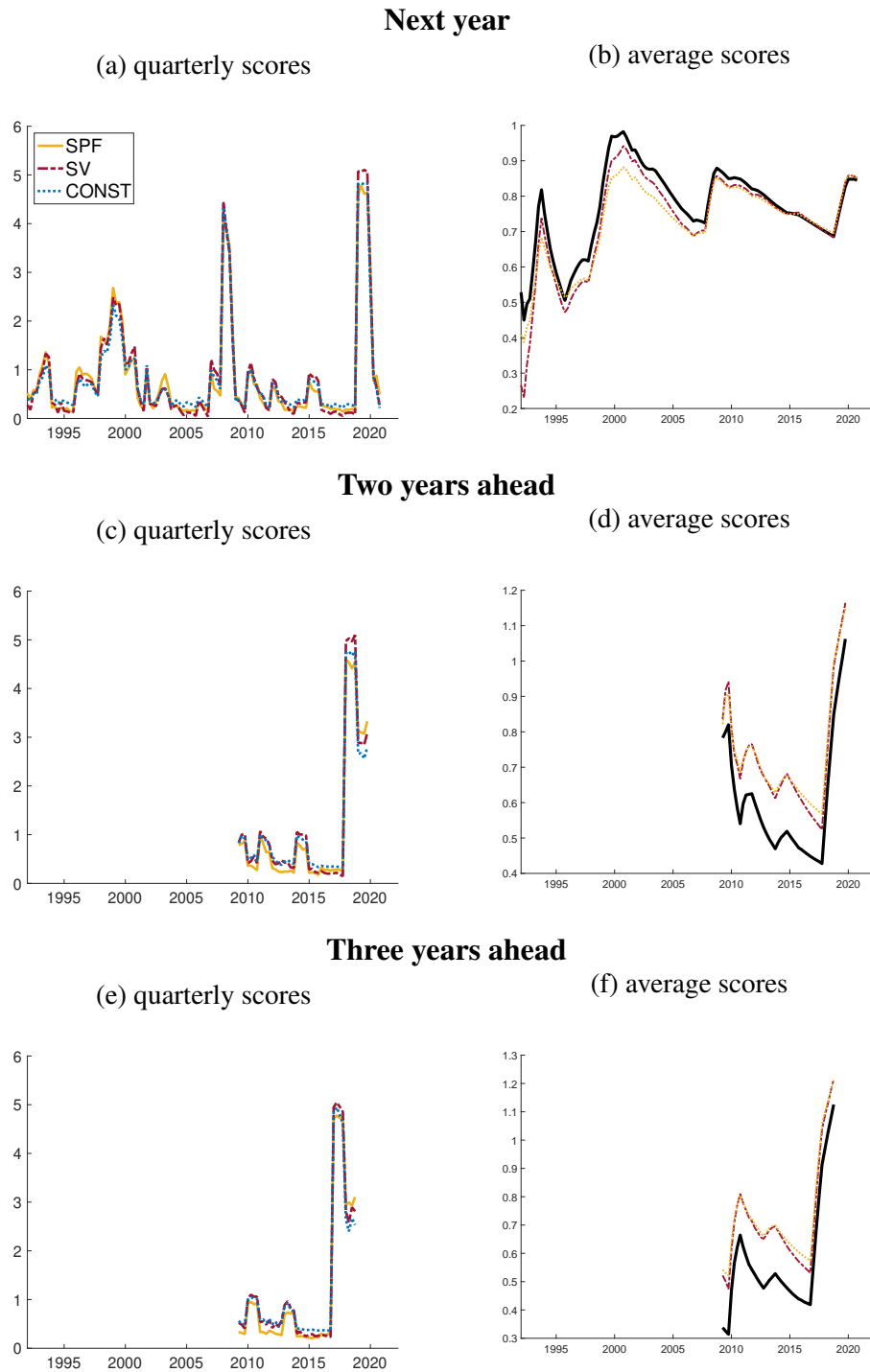
Figure 4: DRPS of models and SPF for annual forecast bins
