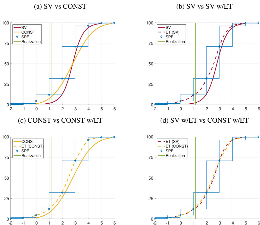
Figure 2: Cumulative distribution functions with and without tilting in 2007Q3
