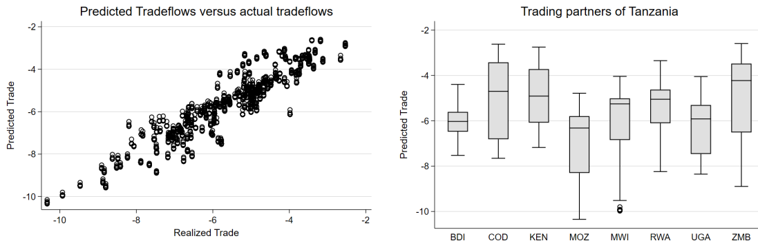
(a) Predicted against realized trade flows
