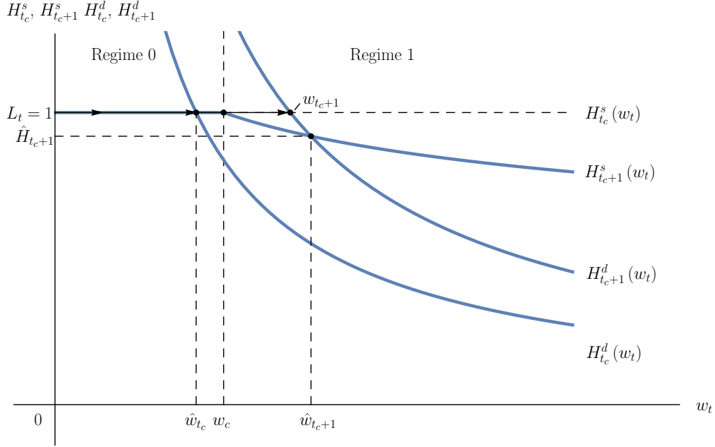
Figure 4.3: The Switch between Regime 0 and 1.
