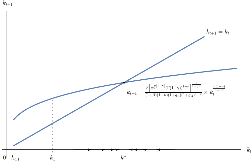
Figure 4.2: The Dynamical System under Regime 1.
