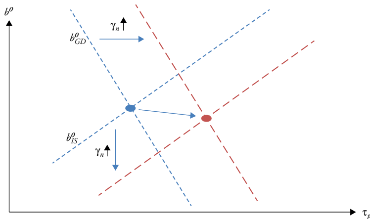
Figure 1 The curves b^o_{IS} and b^o_{GD} and their reactions to an increase in \gamma_n
