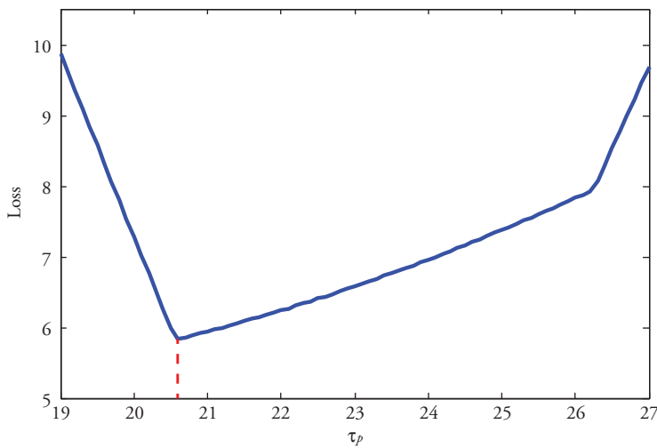
Figure 2 The function \tau_p \mapsto L_\omega(\tau_p) , given \omega = 0.50
