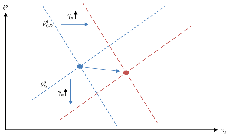
Figure 1 The curves b_{IS}^o and b_{GD}^o and their reactions to an increase in \gamma_n
