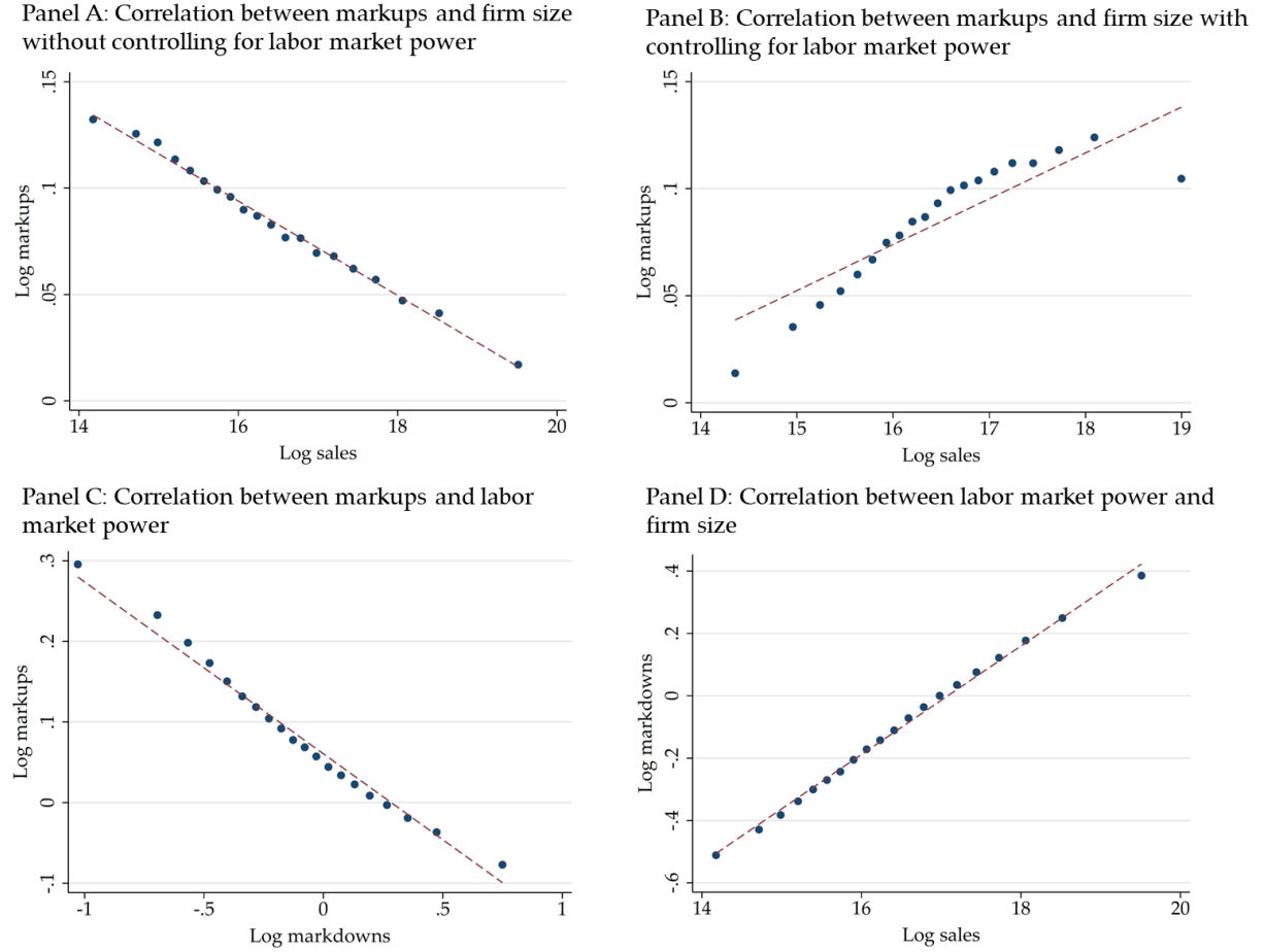
FIGURE 1 – Binned scatter plots from firm-level regressions. Panel A (B) shows results from projecting markups on firm size without (with) controlling for firms' markdowns. Panel C shows results from regressing markups on markdowns. Panel D shows results from regressing markdowns on firm size. All regressions control for industry and year fixed effects. German manufacturing sector data. 1995-2016. 242,303 firm-year observations.
