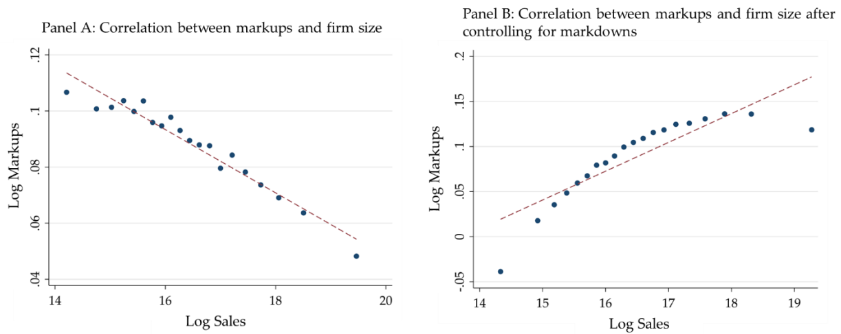
FIGURE D.5 – Binned scatter plots from firm-level regressions of log markups on log sales while controlling for year and four-digit industry fixed effects. Panel A (B) shows results without (with) controlling for firms' markdowns. German manufacturing sector data. 1995-2016. 224,821 firm-year observations.
