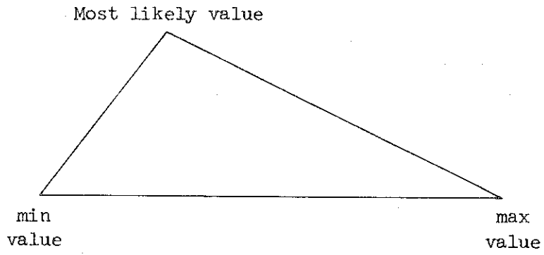
Figure 5.--Triangular Distribution
