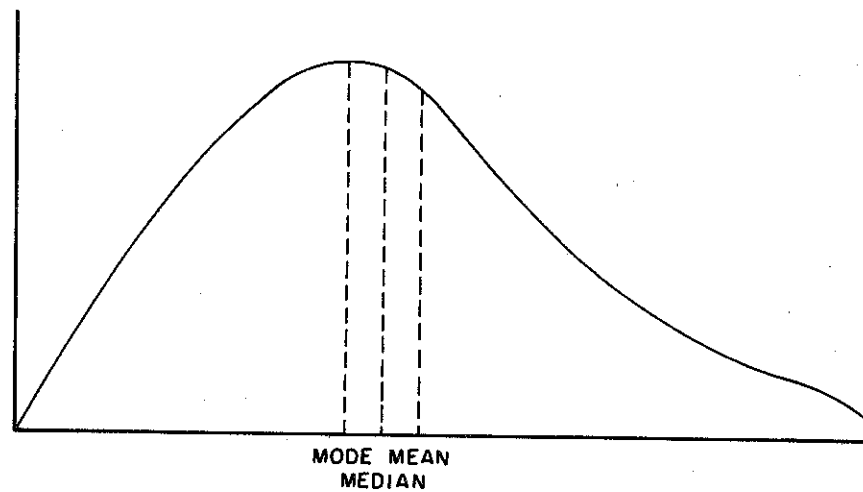
Figure 6.--Lognormal Distribution
