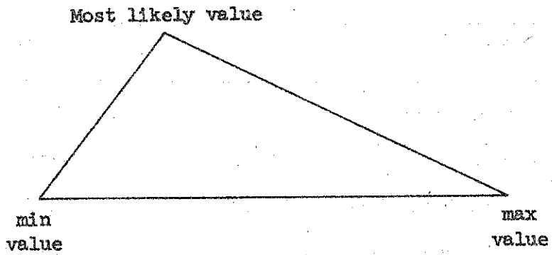
Figure 4.--Triangular Distribution
