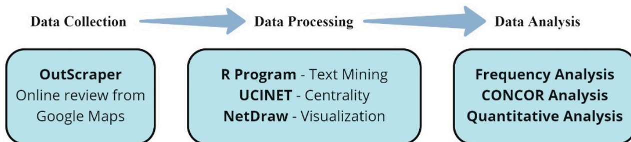
Figure 1. Research Procedures.
