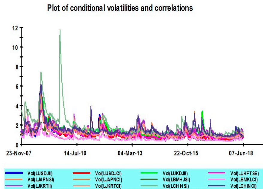
Figure 4. Conditional volatility.
