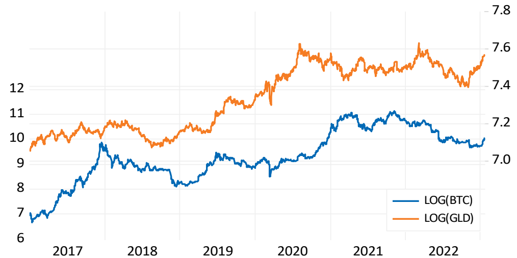
Figure 1. Price dynamics of Bitcoin and gold (in logarithmic scale) from 2 January 2017 to 20 January 2023.
