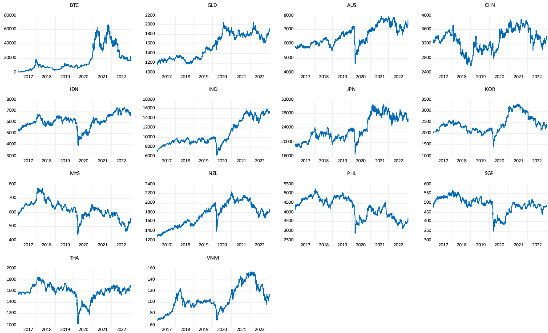
Figure 2. Prices dynamics of Bitcoin, gold, and ASEAN+6 stock indices.
