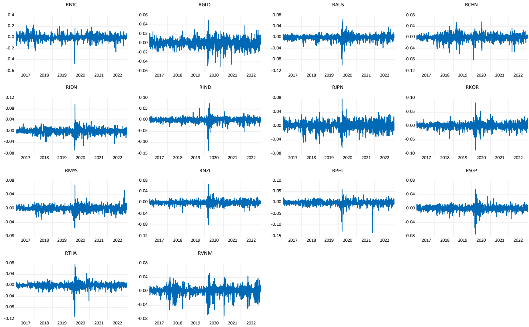
Figure 3. Returns of Bitcoin, gold, and ASEAN+6 stock indices.
