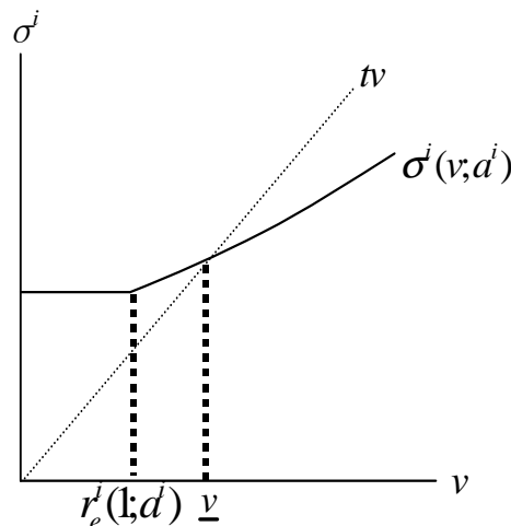
Figure 2: \sigma^i Function
