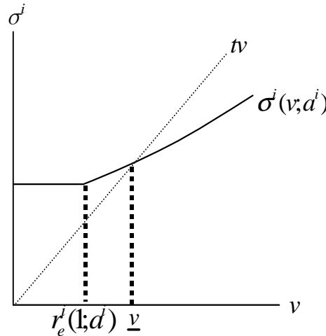
Figure 2: \sigma^i Function
