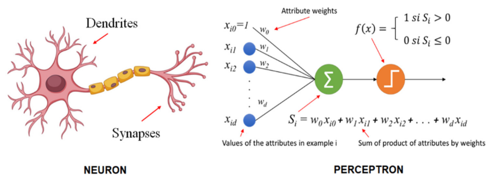
Figure 12. A physical Neuron (left) and its computational analogy; a Perceptron (right) (Image by: Liu, X.; 2021. “How to Train AI using Bitcoin”) (Liu 2021b).
