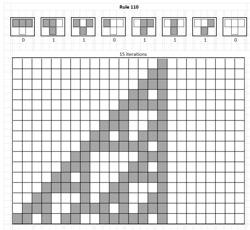
Figure 7. Diagram of Rule 110 Elementary cellular automaton and its consequent evolution. The rule specifies the next color in a cell, depending on its color and its immediate neighbors. The rule is illustrated above together with the evolution of a single black cell it produces after 15 steps. (Image reproduced in Microsoft® Excel® based on Rule 110 by S. Wolfram’s A New Kind of Science ) (Wolfram 2002).
