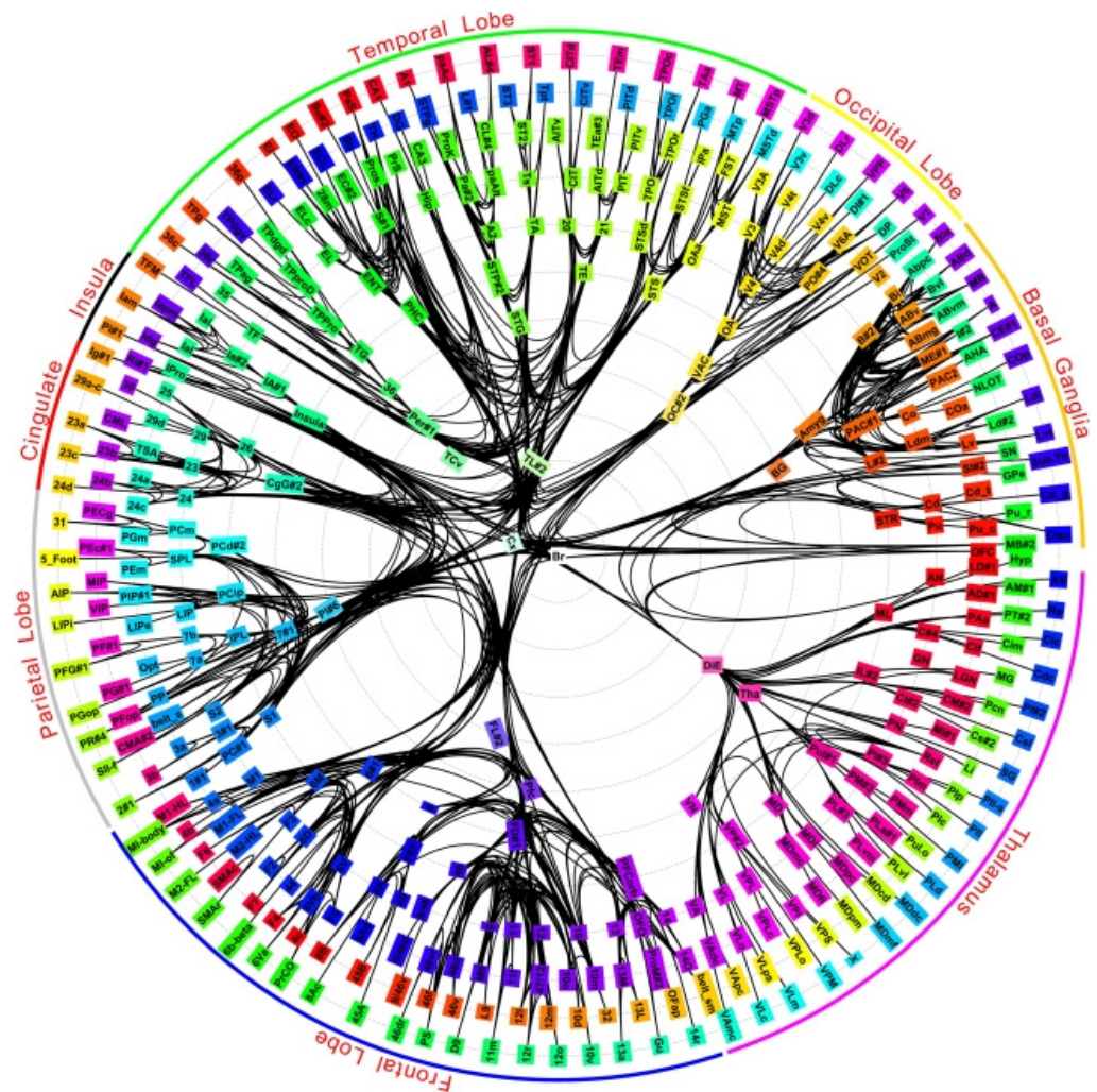
Figure 5. “The Mandala of the Mind”: The long-distance network of the Macaque monkey brain, spanning the cortex, thalamus, and basal ganglia, showing 6602 long-distance connections between 383 brain regions. (Image by: Bernard Goldbach. “Network architecture of the long-distance pathways in the macaque brain”). (CC BY 2.0) ( Modha and Singh 2010 ).
