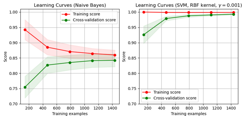
Figure 13. Learning curves (naïve Bayes) and cross-validation scores in existing models can never go over 100% (Image created with scikit 0.24.2. 2021. “Plotting Learning Curves”) (Scikit 2021).
