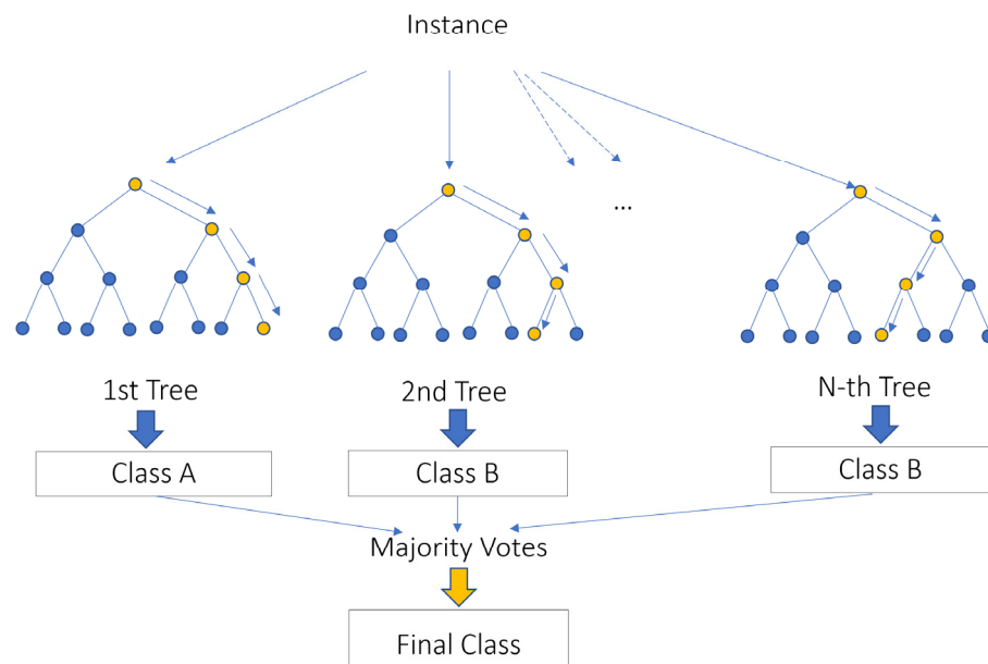
Figure 3. A random decision forest graph. The above illustration shows three decision trees and a classification obtained from each of them. The final prediction is based on majority voting and will be “Class B” in the above case (Image reproduced based on the work from Venkata, J. 2020. “Random Forest Template for TIBCO Spotfire”. CC BY-SA 4.0) (Venkata 2020).
