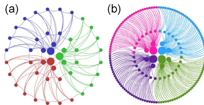
Figure 6. Representations of Mandala Type networks and their node connections (a) type A, generated with parameters b = 2 , n_1 = 3 and \lambda = 2 . (b) type B, generated with parameters b = 4 , n_1 = 4 and \lambda = 2 . (Image by: Sampaio, F.; Moreira, C.; Andrade, A.; et al.; 2015. “Mandala Networks: ultra-small-world and highly sparse graphs”) (Sampaio et al. 2015).
