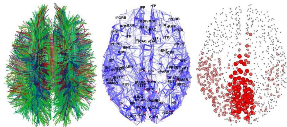
Figure 4. Representation of the human connectome. Images show the fiber architecture of the human brain as revealed by diffusion imaging (left), a reconstructed structural brain network (middle), and the location of the brain’s core, its most highly and densely interconnected hub (right). The image on the left is courtesy of Patric Hagmann, University of Lausanne; the middle and right panels are from Hagmann et al. (Hagmann et al. 2008), (Sporns 2010).
