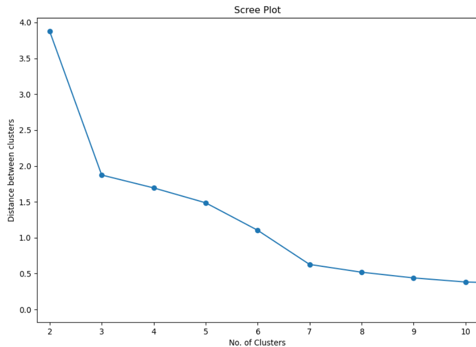
Figure 1. Scree plot for HAC.
