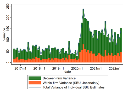
Figure 6. A variance decomposition of the firm-level sales growth rate forecasts. Notes: Calculated using monthly samples of firm-level five-point forecast distributions for sales growth rates. The green rectangles report the activity-weighted between-firm variance of the four-quarter-ahead mean forecasts. The red rectangles report the activity-weighted average within-firm variance of the forecast distributions. The sum of these two components equals the overall variance of the forecasts in data pooled over all firms in a given month. See Equation (1) in the main text for an explicit statement of the variance decomposition. Data through May 2022. Source: Survey of Business Uncertainty conducted by the Federal Reserve Bank of Atlanta, Stanford University, and the University of Chicago Booth School of Business.
