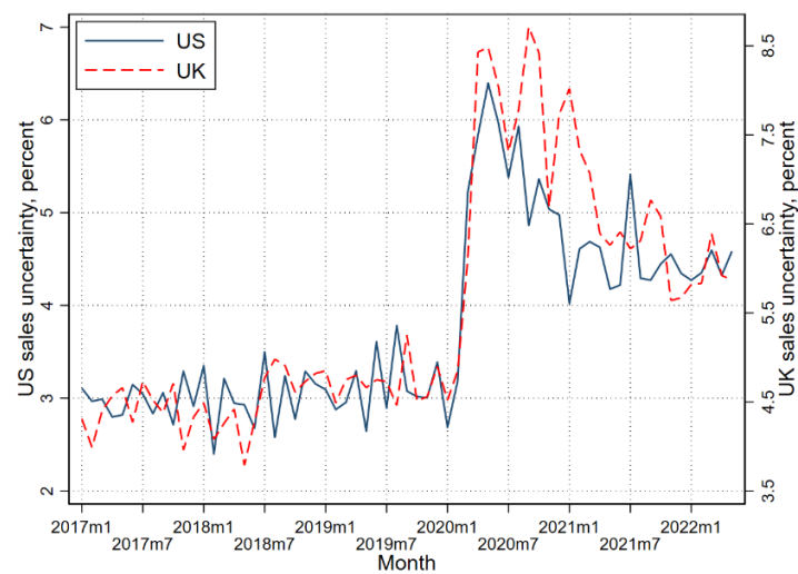
Figure 1. SBU (United States) and DMP (United Kingdom) uncertainty indexes. Note: SBU and DMP data through May 2022. Sources: US firm-level sales growth rate uncertainty from the Federal Reserve Bank of Atlanta’s Survey of Business Uncertainty (in partnership with Chicago Booth and Stanford University). UK firm-level sales growth rate uncertainty from the Bank of England’s Decision Makers Panel (in partnership with Nottingham University).
