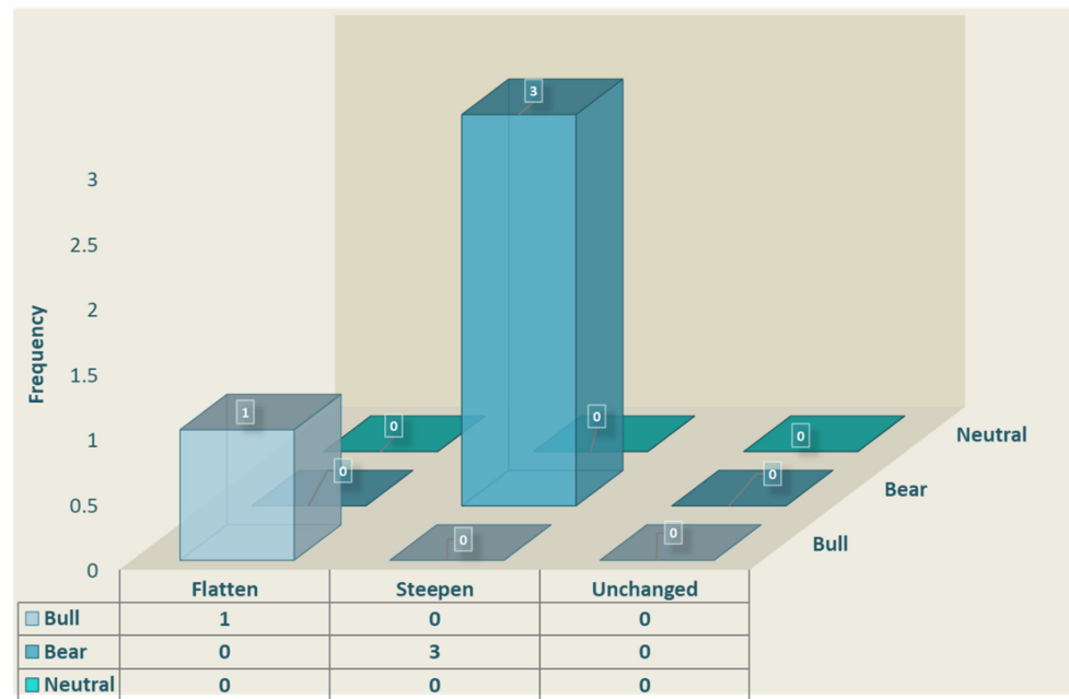
Figure 10. Weekly yield curve patterns on 20 March 2020 (last 4 weeks). Source: Bloomberg yields, own computation of yield curve patterns.
