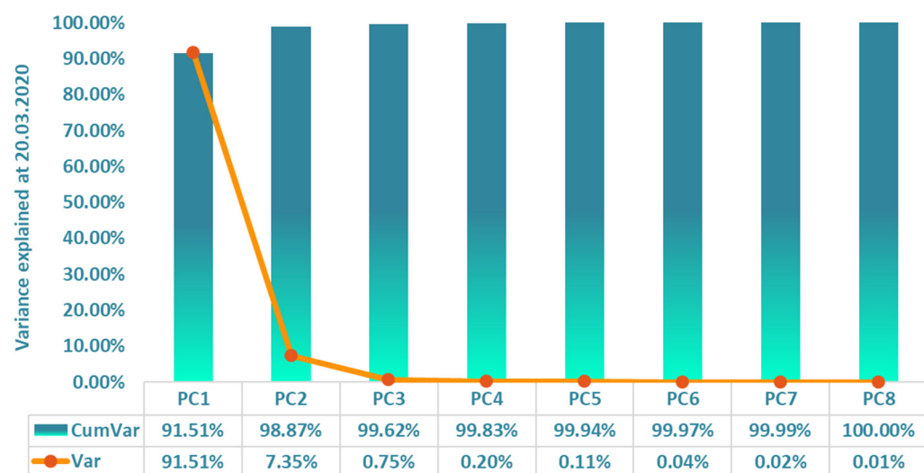
Figure 7. Yield curve variability explained by principal components on 20 March 2020. Source: Bloomberg, own computation of PCs with the use of a VBA add-in developed by Leonardo Volpi.
