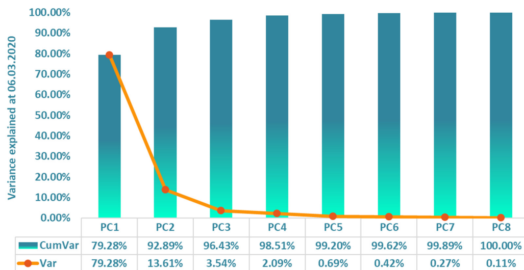
Figure 6. Yield curve variability explained by principal components on 6 March 2020. Source: Bloomberg, own computation of PCs with the use of a VBA add-in developed by Leonardo Volpi.
