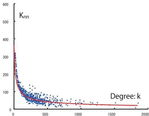
Figure 5: Degree Correlation
