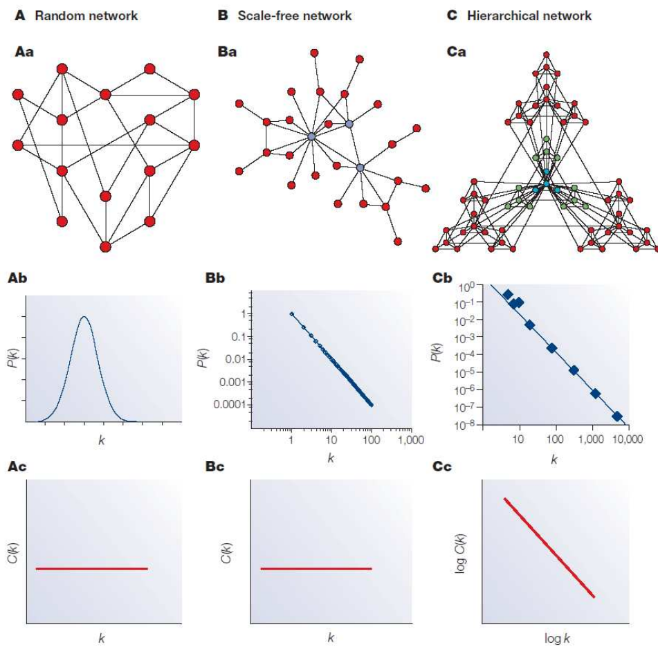
Figure 1: Network Structures
