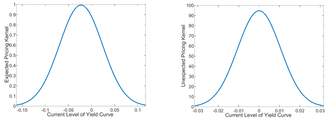
Figure 2. Expected (9) and Random Components of the SDF (10).
