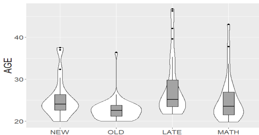
Figure 4: AGE by study group
