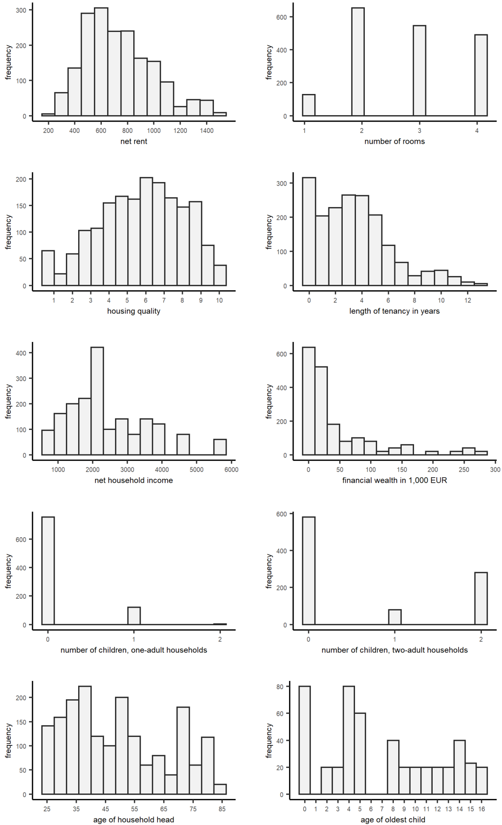
Figure A5: Simulation data: histograms
