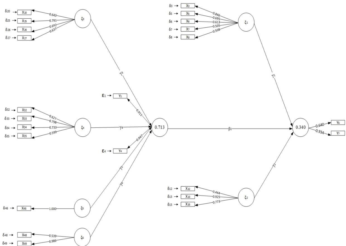
Figure 4. Indicators of outer loading that passed the convergent validity.
