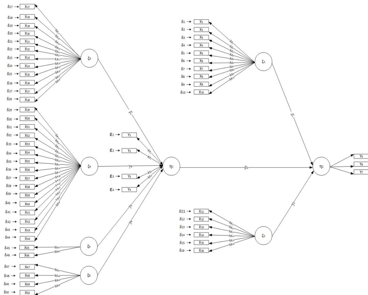
Figure 3. Path diagram of the SEM model.
