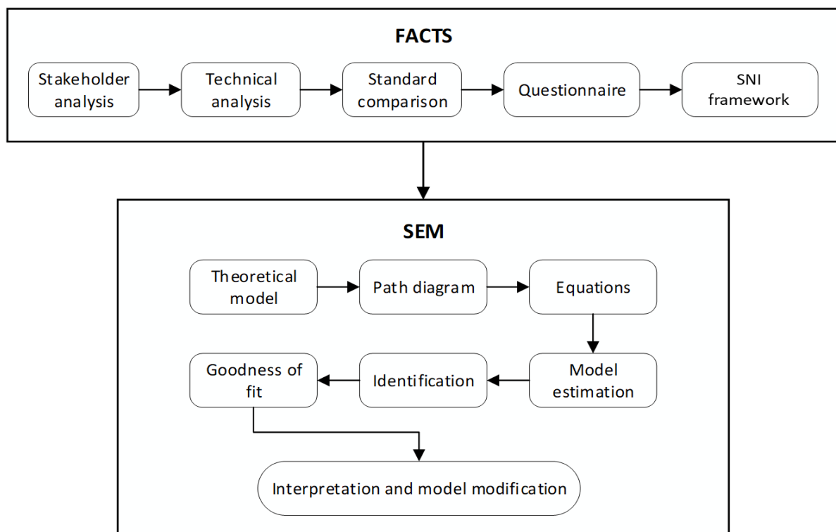
Figure 1. Sequential mixed methodology of the study.
