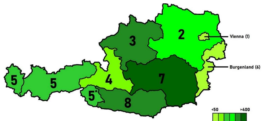
Figure 1. The number of farmer shops by region according to their postal code.
