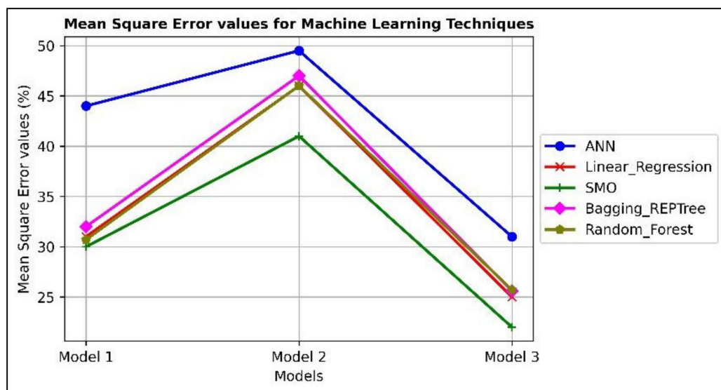
Figure 4. ML techniques mean square error.
