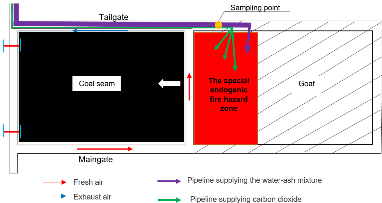
Figure 9. Diagram of the examined area with the method of administering substances limiting the occurrence of an endogenic fire to the hazard zone.
