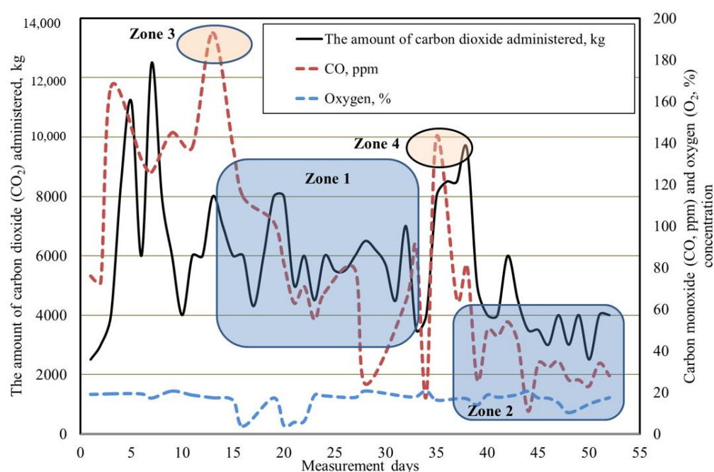
Figure 10. Temporary changes of carbon monoxide (CO) and oxygen (O 2 ) concentrations in the mine atmosphere while inerting the goaves with carbon dioxide (CO 2 ).
