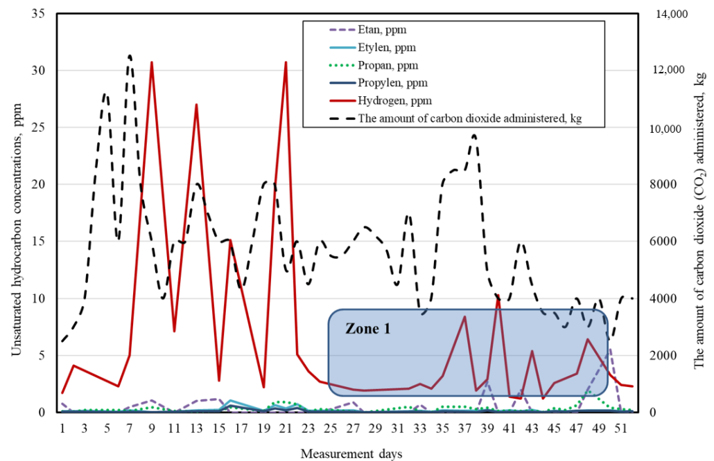
Figure 11. Temporary changes of unsaturated hydrocarbon concentrations in the mine atmosphere while inerting the goaves with carbon dioxide ( \text{CO}_2 ).
