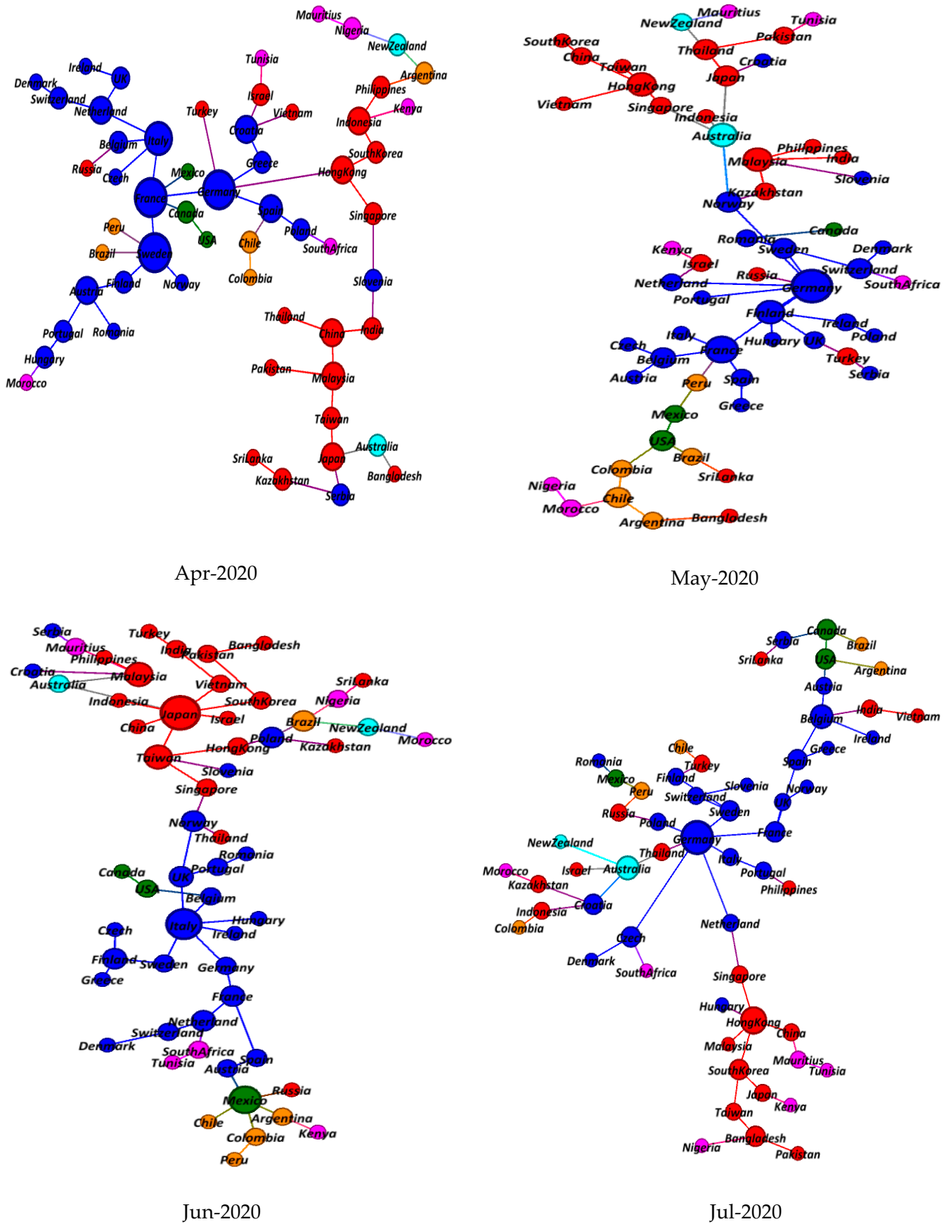
Figure 3. Comparison of dynamic MSTs of the world stock market network from April 2020 to July 2020.
