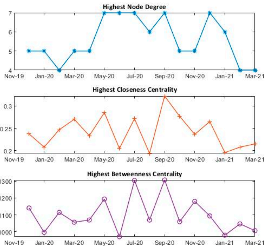
Figure 6. Highest centrality measures for each of the MSTs of the world stock network.
