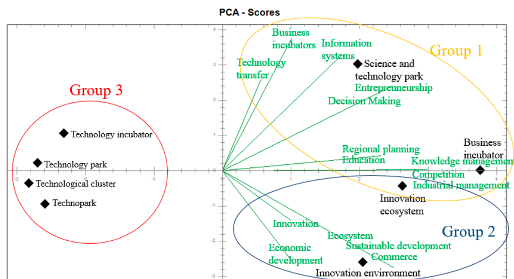
Figure 7. Biplot PCA Scores.
