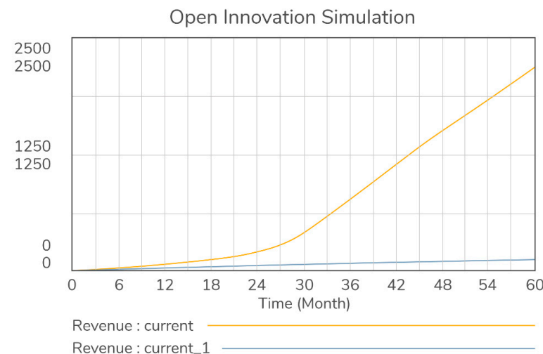
Figure 5. The OI simulation with OI variables (current) and without OI variables (current_1).
