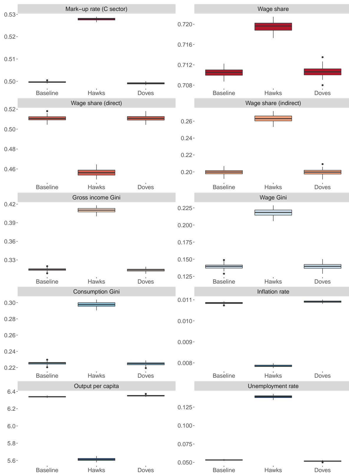
Figure 12: Comparison of experiments (monetary policy rules)
