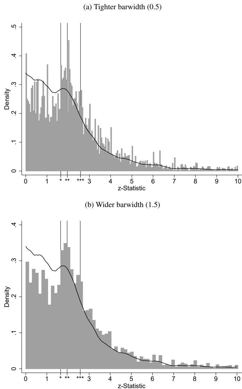
Figure A1: Distributions of z-statistics for initial submissions - Alternate barwidths
