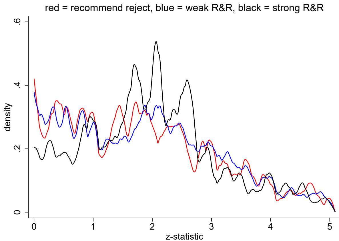
Figure A3: Smoothed distributions of z-statistics reviewer recommendation
