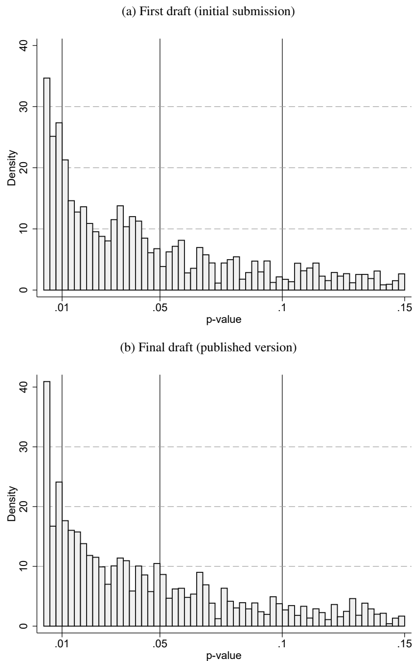
Figure A10: De-rounded distributions of p-values by draft versions of accepted manuscripts
