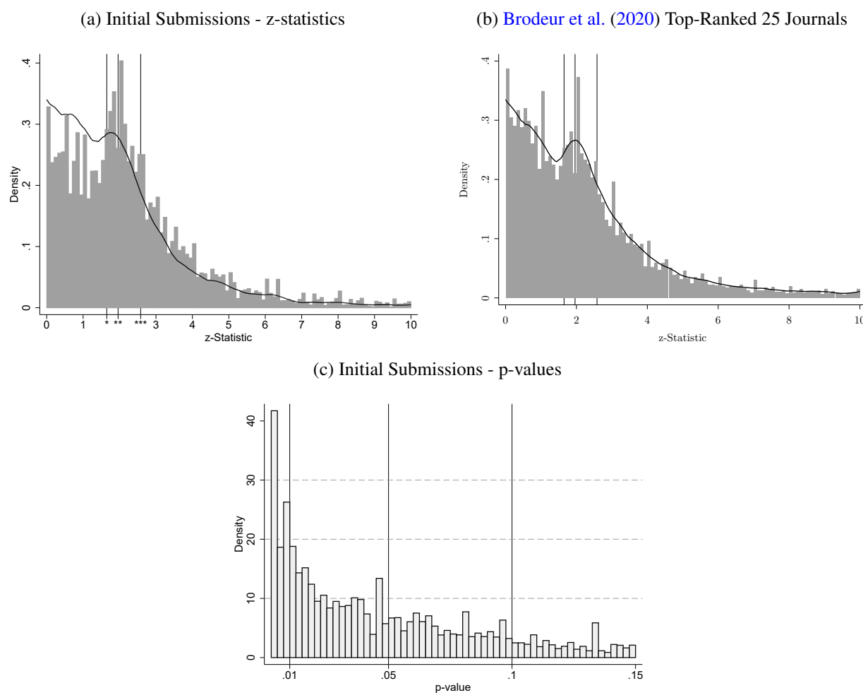
Figure 2: Distributions of z-statistics and p-values for initial submissions vs. z-statistics from Brodeur et al. (2020)
