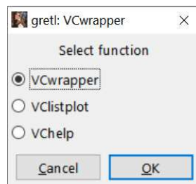
Fig. 6: VC menu
