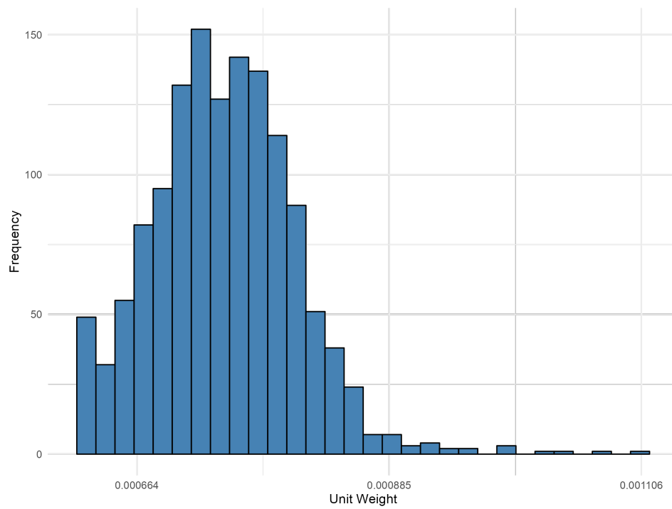
Figure A3: Histogram of Unit Weights in Synthetic Diff-in-Diff Approach
