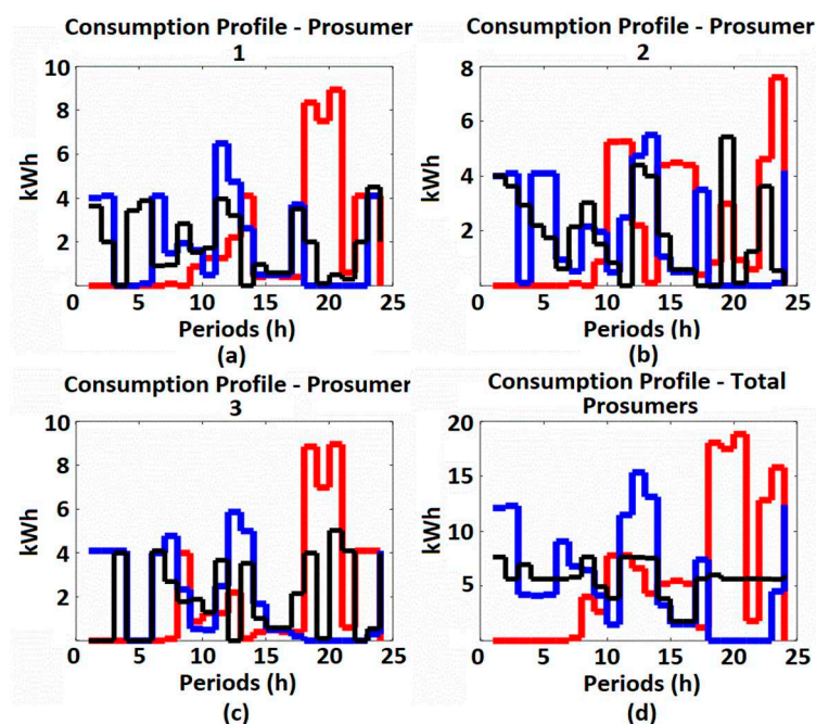
Figure 3. Habitual consumption profile and profiles of optimal consumption without and with the improvement of the LF. (a) Consumption profiles for prosumer 1; (b) Consumption profiles for prosumer 2; (c) Consumption profiles for prosumer 3; and (d) Consumption profiles for all prosumers.
