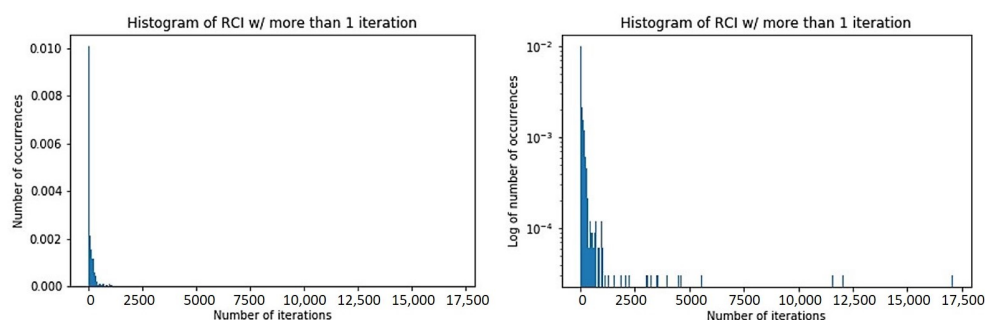
Figure 9. Histogram of the number of iterations for the convergence of each RCI process that needed more than one iteration to find a solution. (Left): Linear scale. (Right): Logarithmic scale.
