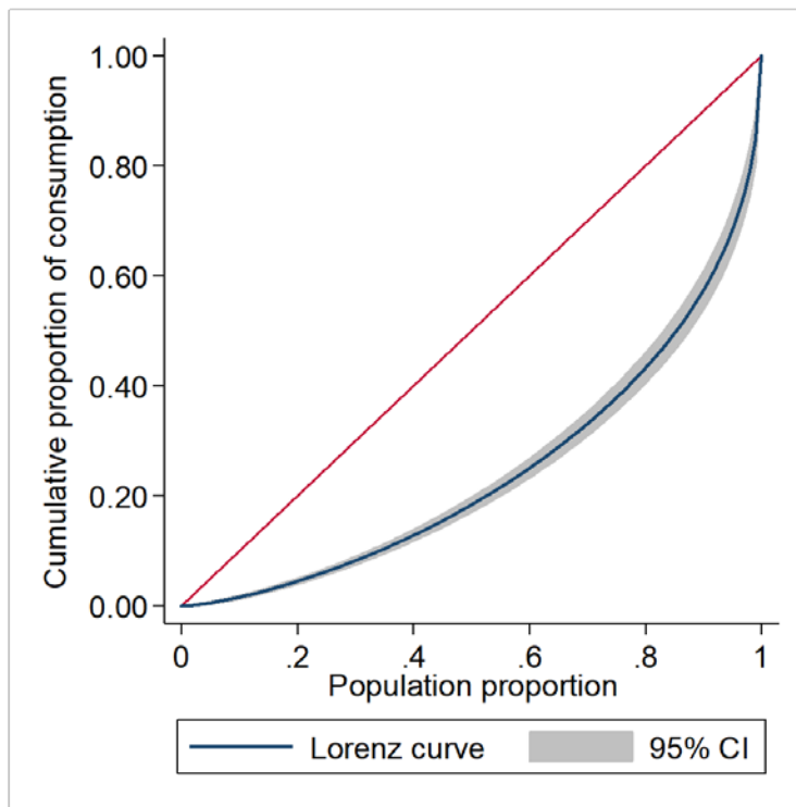
Figure 6: Lorenz curves
