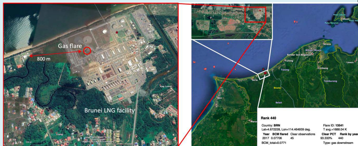
Figure B2: Example gas flare in Brunei, member of ASEAN, as observed by VIIRS satellite
