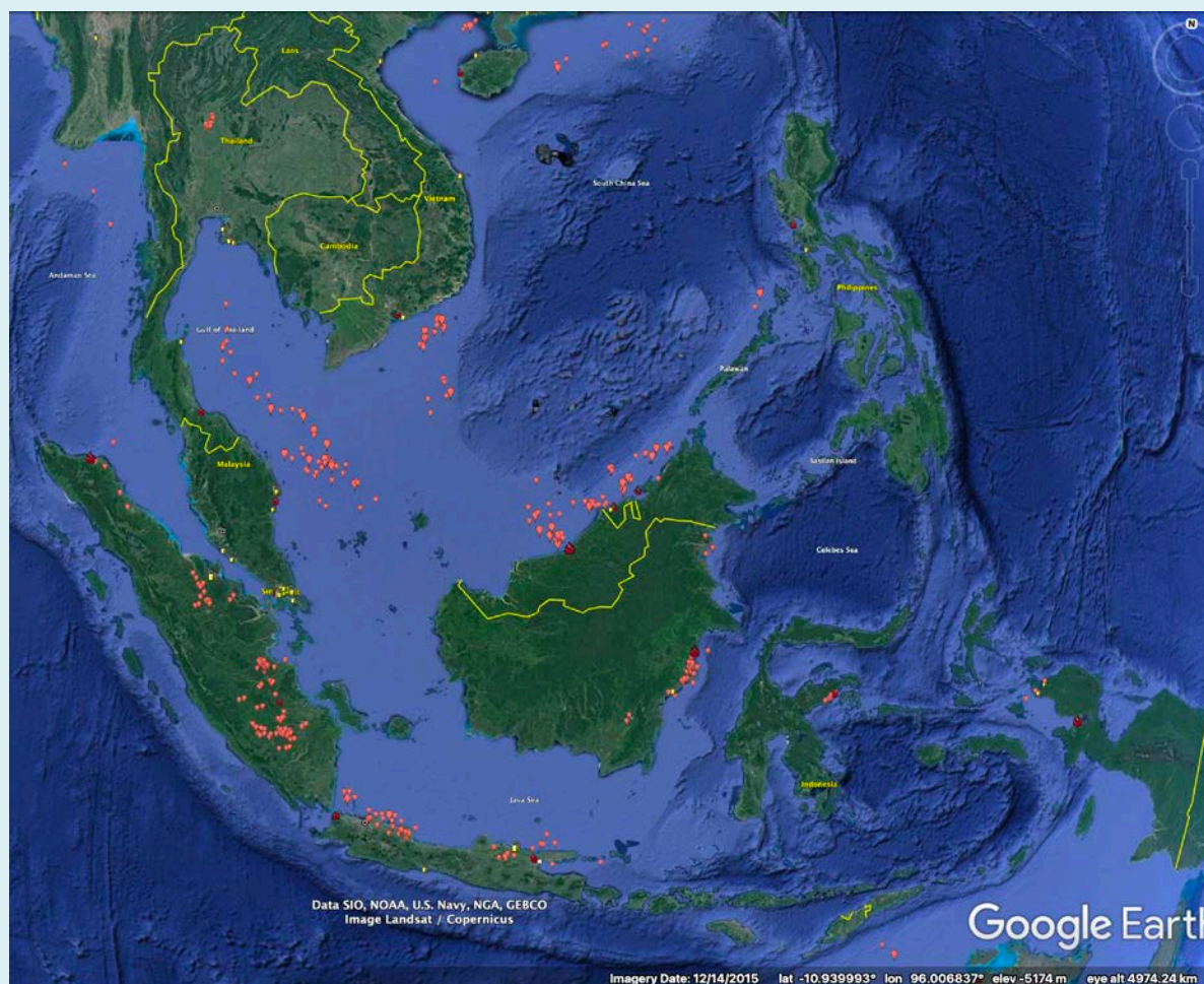
Figure B1: Individual natural gas flares in ASEAN countries as observed by VIIRS satellite
