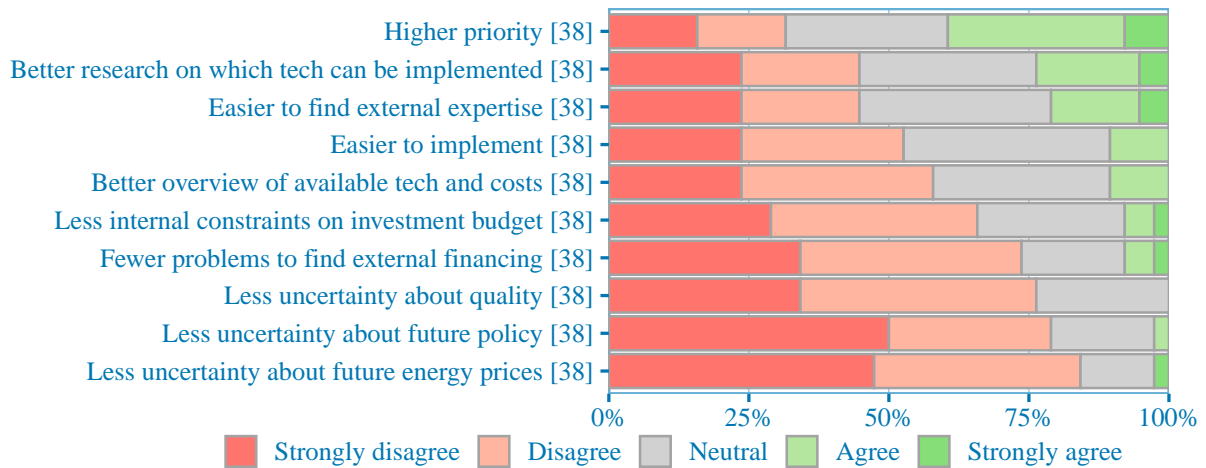
Figure 8: POLICY EVALUATION.
