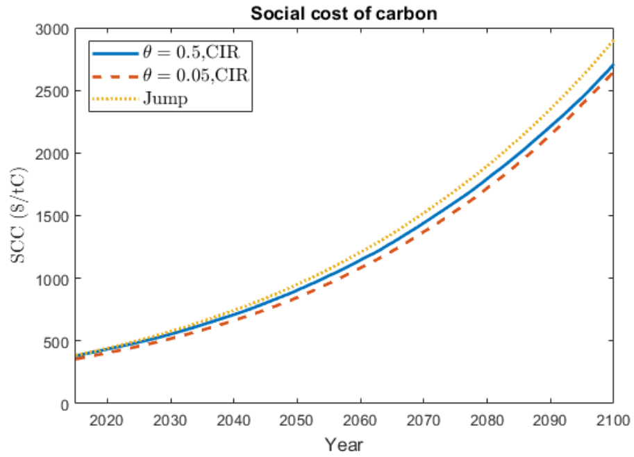
Figure 24: Social costs of carbon in the BAU scenario when \bar{\lambda}_t either jumps immediately (“Jump”) or follows an CIR process (“CIR”) under \sigma_\lambda = 0 and different speed \theta .
