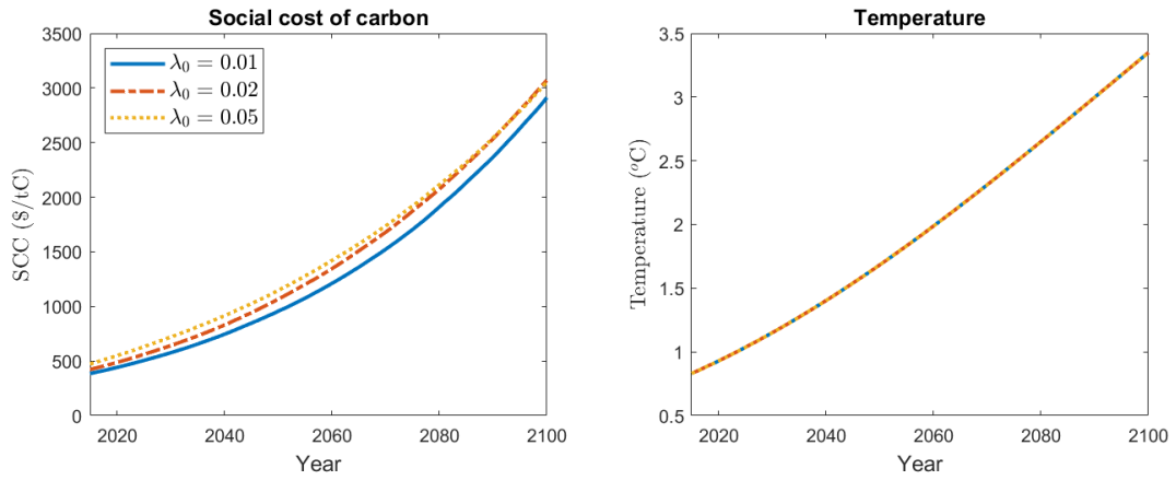
Figure 33: Social cost of carbon (US dollar per ton of carbon, or $/tC) and mean global surface temperature (°C) in the business-as-usual (BAU) scenario from 2015 to 2100 under \lambda_0 = 0.01, 0.02 , and 0.05 , where \bar{\lambda}^{(H)} = 2\bar{\lambda}^{(L)} .
