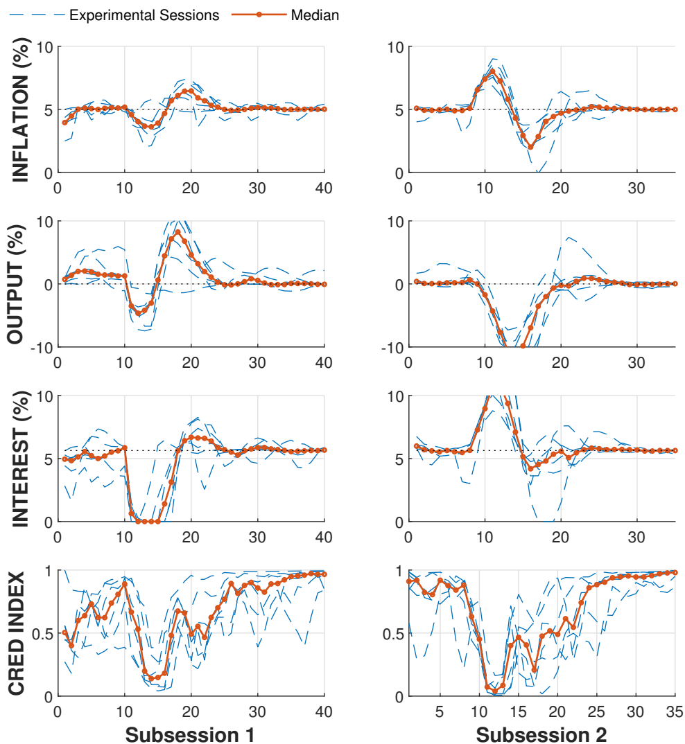
Figure 4: Inflation, output and interest rate dynamics in Tr. PLT-G
