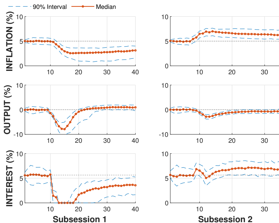
Figure 9: Inflation, output and interest rate dynamics in IT treatment in NK-SL
