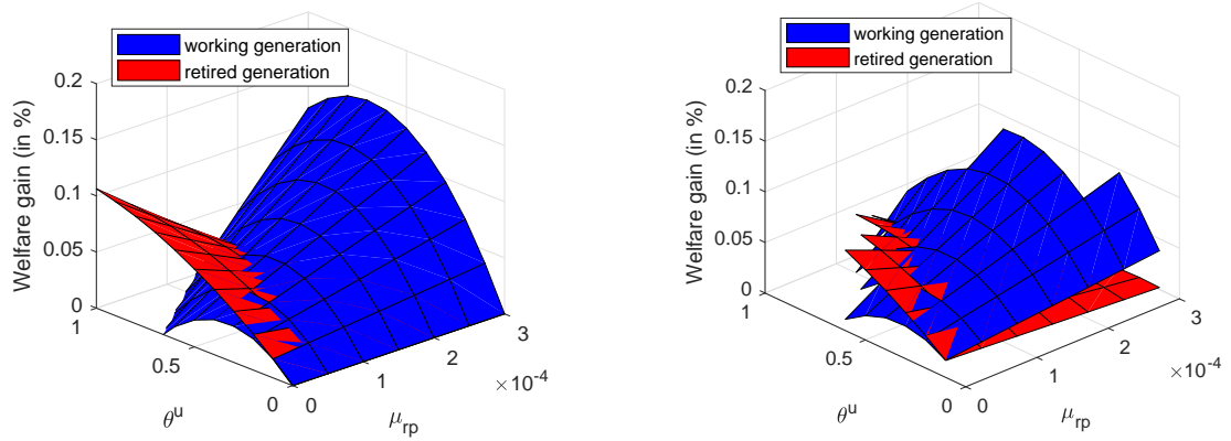
Figure 9: Welfare gain for different allocations of the infinite horizon IGR contract ( \theta^u ) and different risk premia ( \mu_{rp} ). The left panel presents the positive welfare gains of the current working generation and future generations and of the current retired generation. The right panel presents the welfare gains if these are strictly positive for all current and future generations.
